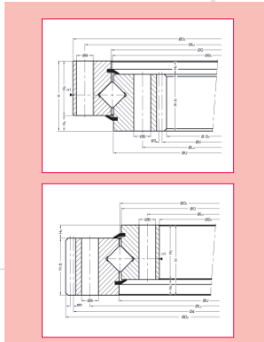
Model Typ 5000 Single-row roller bearing slewing rings
